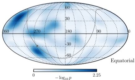
Figure: skymap
