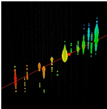
Figure: Track
