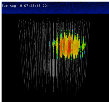
Figure: Cascade
