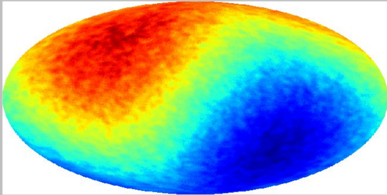
Mollweide view
